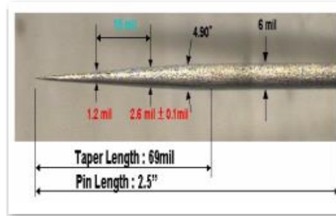
Wire Probe Pin
