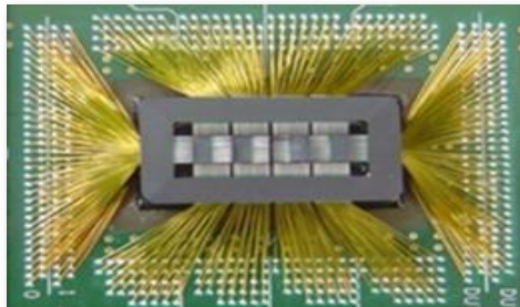
Probe Card for ASIC
