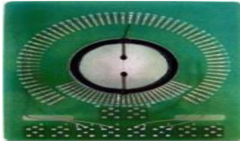
Probe Card for LED
